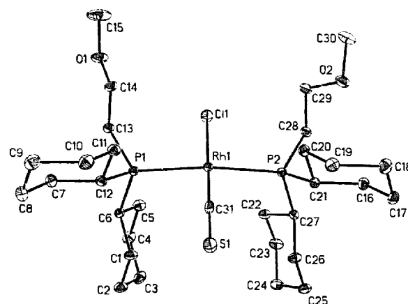
Fig. 2. ORTEP plot of the rhodium complex 5.
